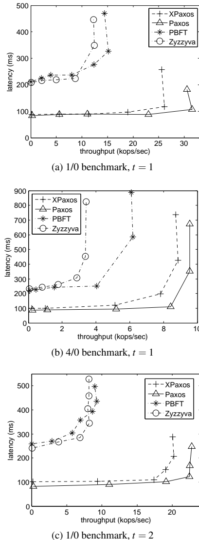
Figure 5: Fault-free performance
